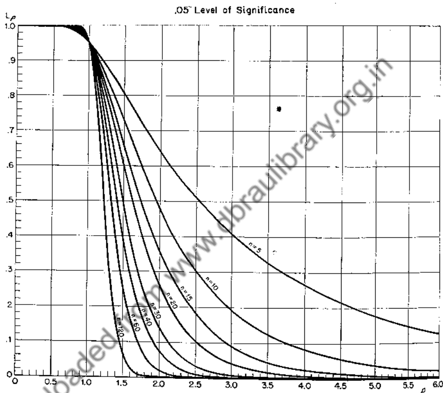
FIG. 8.1.—Operating-characteristic curves for experiments to determine whether a new product (process) is more variable than a standard product (process) of known variability, 0.05 level of significance.
