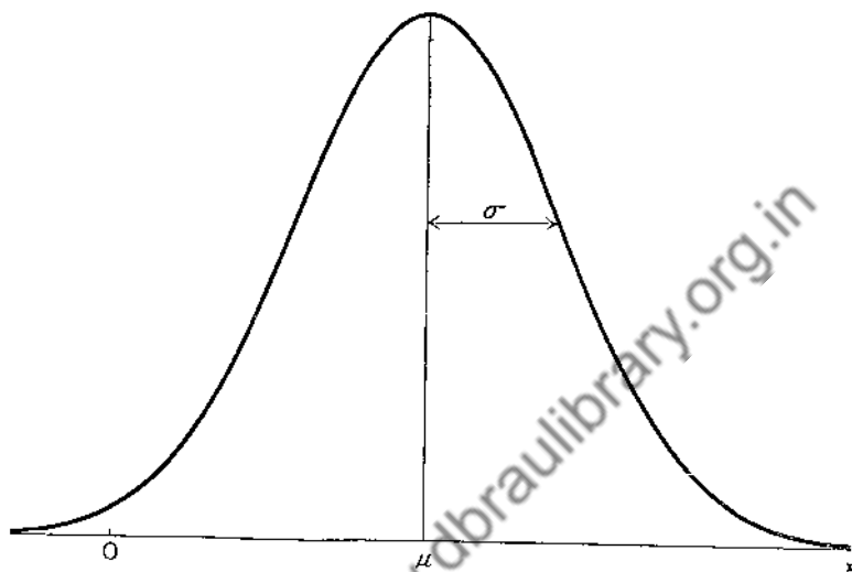
FIG. 1.1.—Normal distribution.
