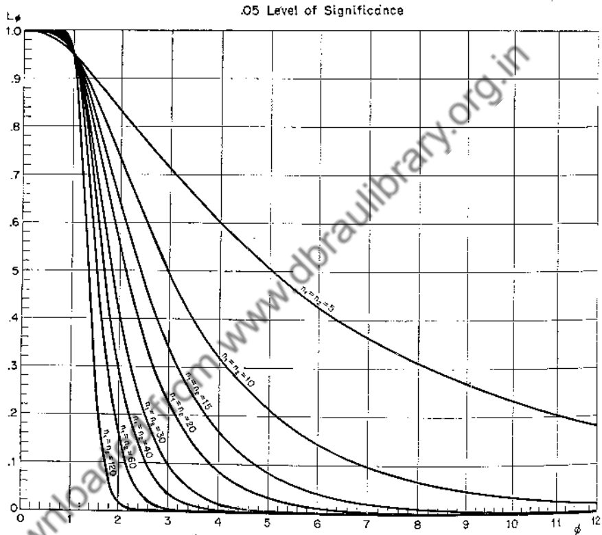
FIG. 8.3.—Operating-characteristic curves for experiments to determine whether a particular one of two new products (processes) is more variable than the other, 0.05 level of significance.
